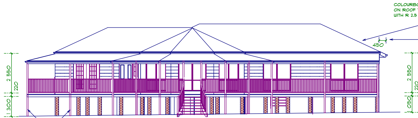
SOUTH ELEVATION
