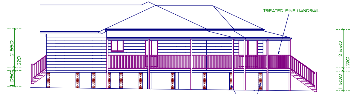
WEST ELEVATION
