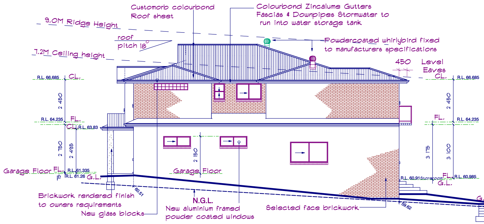
SOUTH ELEVATION (1 : 100) ( Side )
